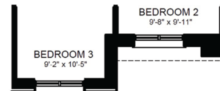
PARTIAL SECOND FLOOR PLAN ELEVATION 'B2'
