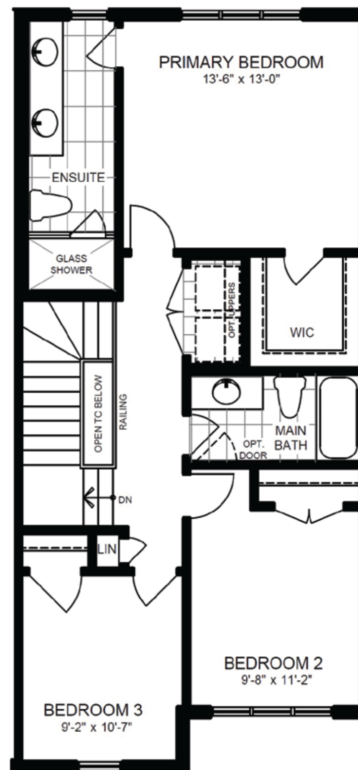
SECOND FLOOR PLAN ELEVATION 'A1'
